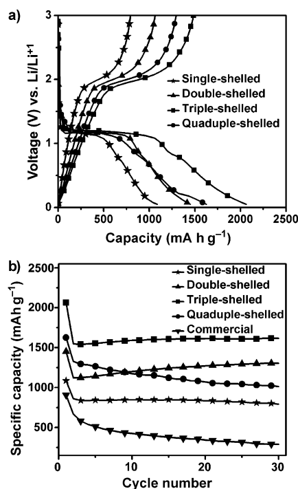
Figure 3. a) First-cycle discharge-charge curves for the multisheled \text{Co}_3\text{O}_4 hollow microspheres at a current density of 50 \text{ mA g}^{-1} between 0.05 and 3.0 V. b) Discharge capacity versus cycle number for the prepared \text{Co}_3\text{O}_4 hollow microspheres and commercial \text{Co}_3\text{O}_4 at a current density of 50 \text{ mA g}^{-1} .
